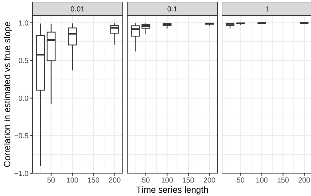
Figure S1: Correlation between the model estimated slope and the true slope as a function of time series length. Each panel represents a different ratio in variability between the slope and intercept.
